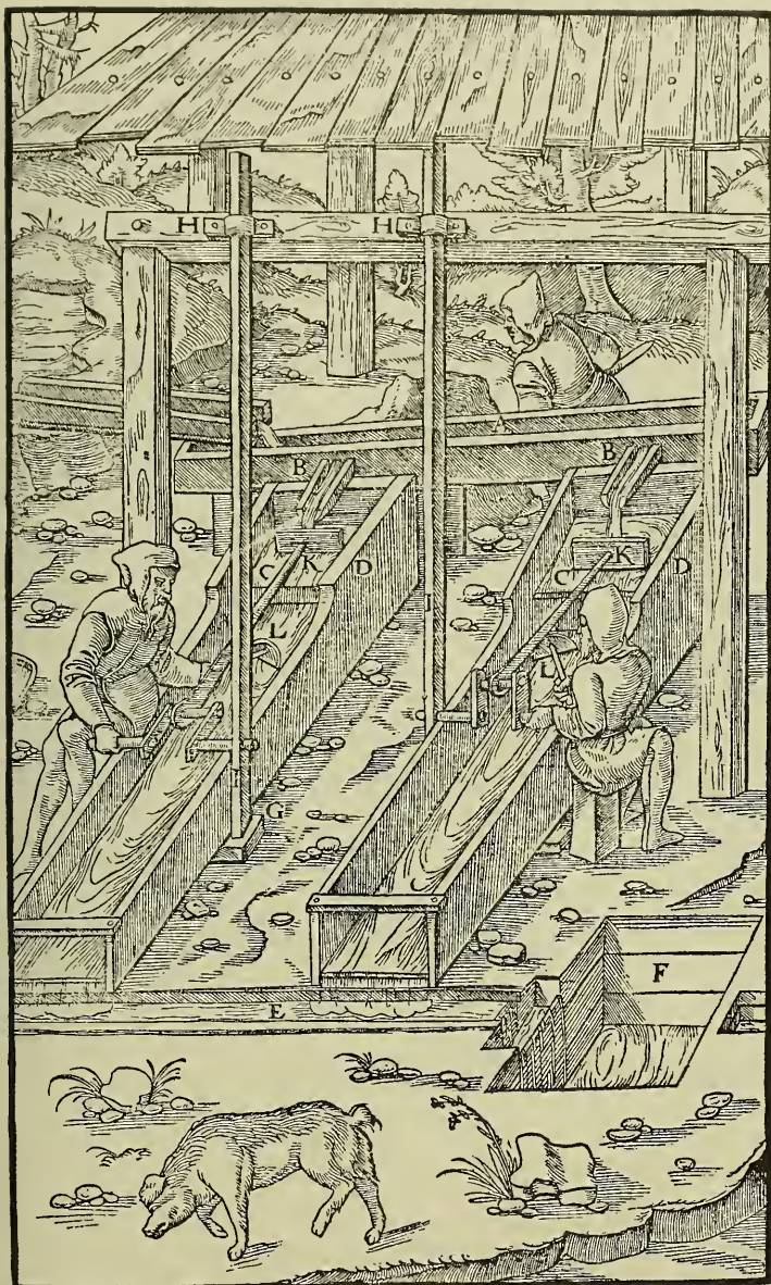
A—UPPER CROSS LAUNDER. B—SMALL LAUNDERS. C—HEADS OF STRAKES. D—STRAKES. E—LOWER TRANSVERSE LAUNDER. F—SETTLING PIT. G—SOCKET IN THE SILL. H—HALVED IRON RINGS FIXED TO BEAM. I—POLE. K—ITS LITTLE SCRUBBER. L—SECOND SMALL SCRUBBER.
