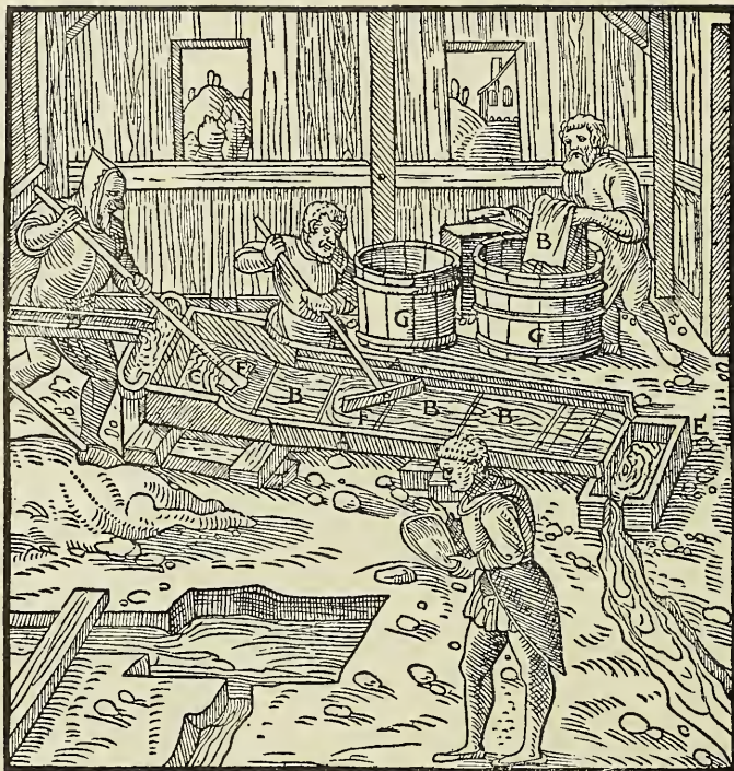
A—BEAMS. B—CANVAS. C—HEAD OF STRAKE. D—SMALL LAUNDER. E—SETTLING PIT OR TANK. F—WOODEN SCRUBBER. G—TUBS.
