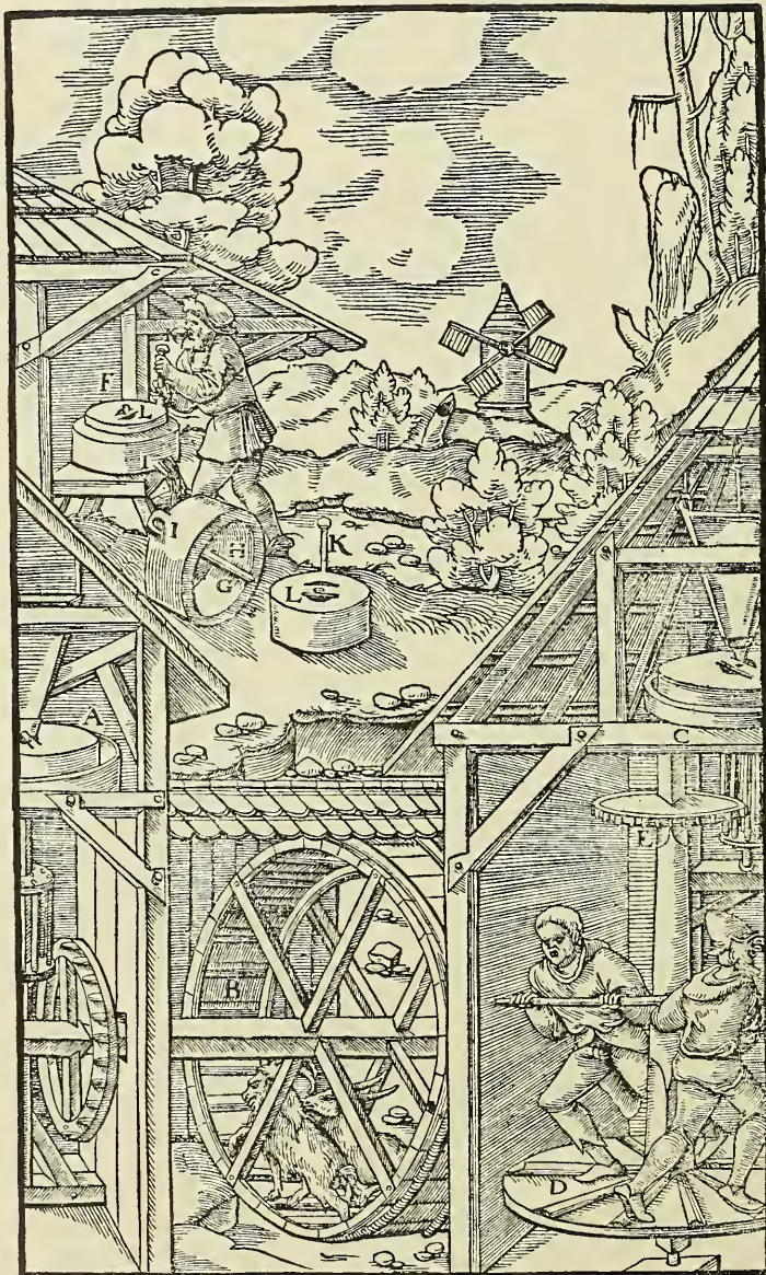
A—FIRST MILL. B—WHEEL TURNED BY GOATS. C—SECOND MILL. D—DISC OF UPRIGHT AXLE. E—ITS TOOTHED DRUM. F—THIRD MILL. G—SHAPE OF LOWER MILLSTONE. H—SMALL UPRIGHT AXLE OF THE SAME. I—ITS OPENING. K—LEVER OF THE UPPER MILLSTONE. L—ITS OPENING.
