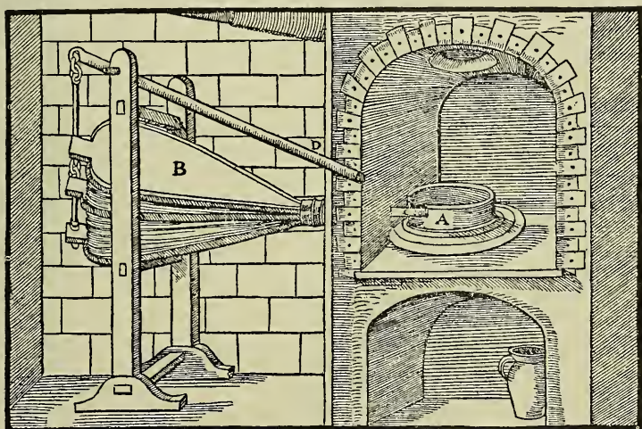
A—IRON HOOP. B—DOUBLE BELLOW. C—ITS NOZZLE. D—LEVER.
