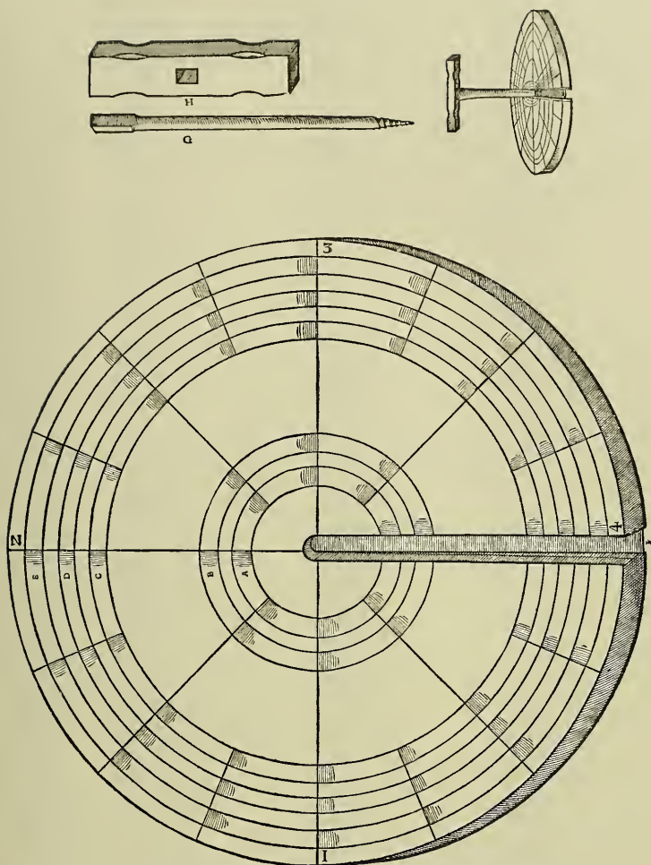
A, B, C, D, E—FIVE WAXED CIRCLES OF THE orbis . F—OPENING OF SAME. G—SCREW. H—PERFORATED IRON.
