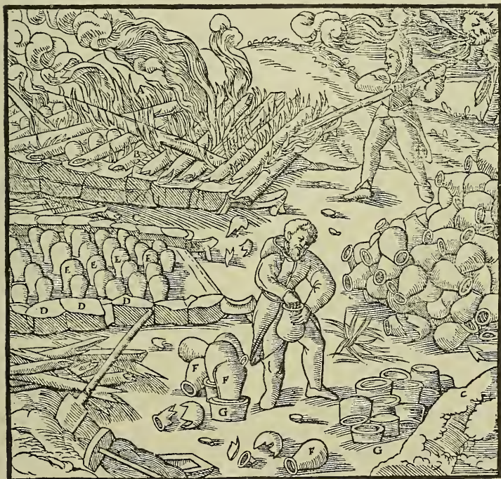
A—HEARTH. B—POLES. C—HEARTH WITHOUT FIRE IN WHICH THE POTS ARE PLACED. D—ROCKS. E—ROWS OF POTS. F—UPPER POTS. G—LOWER POTS.
