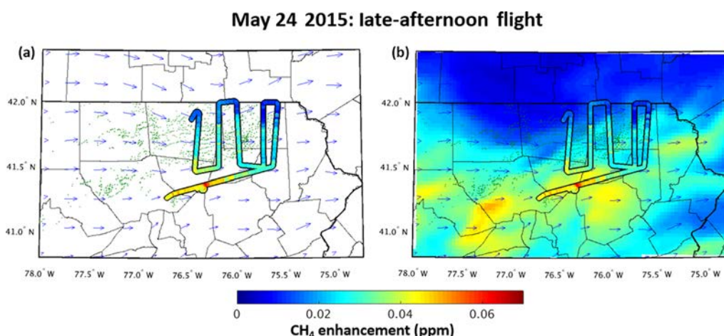
Figure 13. (a) Observed CH 4 enhancement from the late-afternoon flight on 24 May 2015. (b) Observed CH 4 enhancement compared to the model projected CH 4 enhancement from the sum of all sources in the region. The colour scale of observed and projected enhancements is scaled 1 : 1, with matching colours indicating matching values. Modelled wind vectors and CH 4 concentrations are from 700 m model height level.
