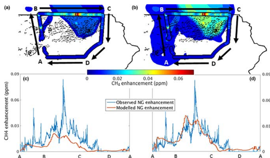
Figure 10. (a) Observed enhancement from unconventional natural gas production overtop projected upstream natural gas enhancements at 700 m from the first loop of the 29 May flight, using an upstream gas emission rate of 0.13 % of production. (c) Direct comparison of the observed natural gas enhancement with the modelled enhancement following the path from A to D using an unconventional emission rate of 0.13 %. (b, d) Same as left figures, except using the optimized upstream emission rate of 0.26 %
