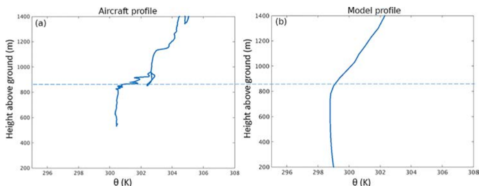
Figure 12. (a) Observed potential temperature profile with height from the first aircraft spiral on the 29 May flight at 17:00 Z. (b) Modelled potential temperature at the location and time at which the aircraft spiral occurred. In both cases, an inversion in the potential temperature profile begins to occur around 850 m.
