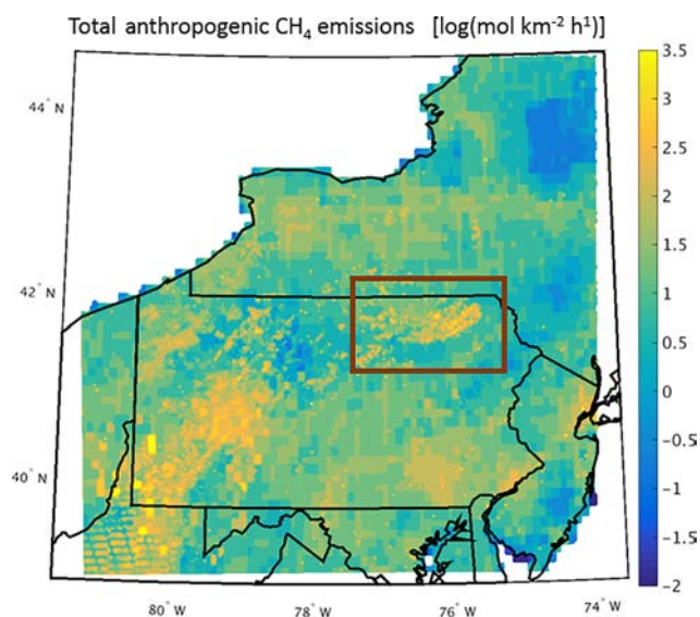
Figure 6. A log-scale contour of the anthropogenic \text{CH}_4 emissions inventory from this study used within the transport model. The red rectangle surrounds the study region where the aircraft campaign took place.
