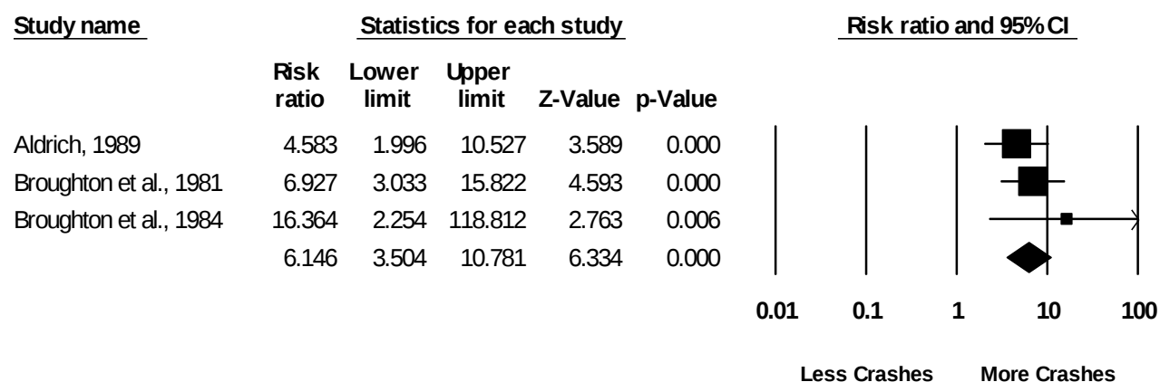
Figure 7: Crash Risk among Individuals with Narcolepsy Compared to Controls (Fixed Effects Meta-Analysis)
