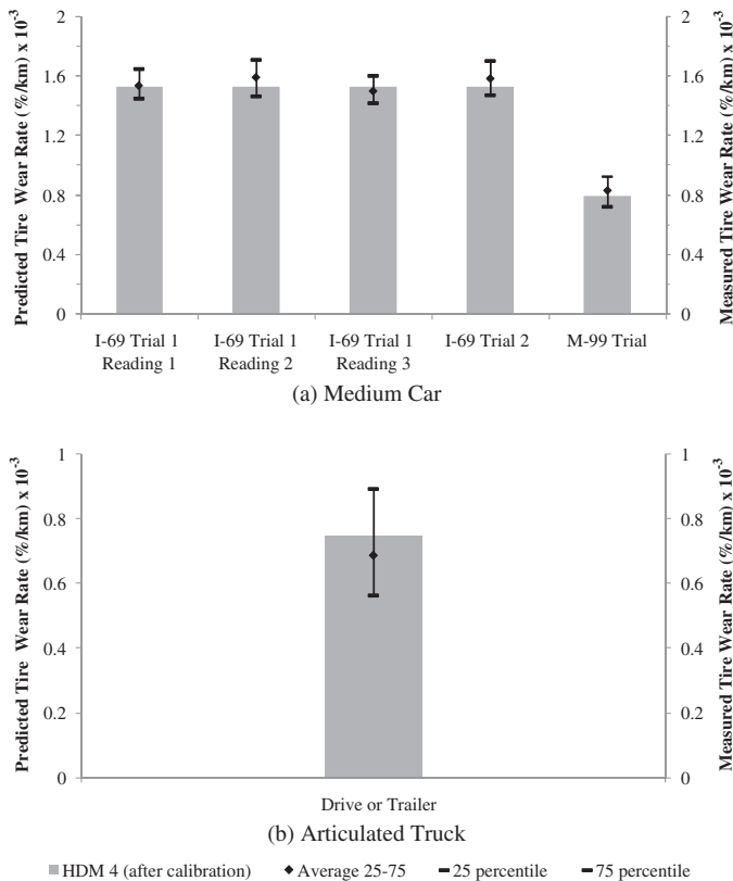
Figure 4-11. Comparison between the calibrated HDM 4 predictions and measurements.
