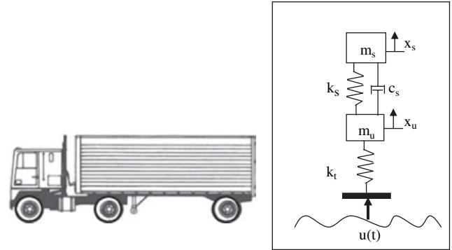
Figure 5-4. Schematic of two-degrees-of-freedom quarter-car vehicle model.
