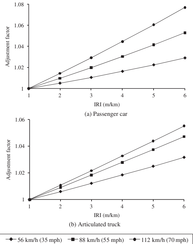
Figure 4-12. Effect of roughness on tire wear estimated using calibrated HDM 4.
