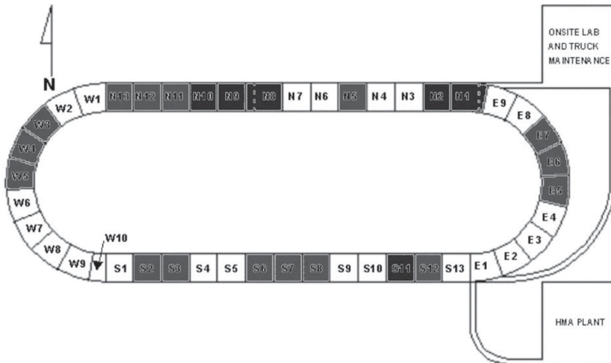
Figure 4-2. NCAT track layout and configuration.
