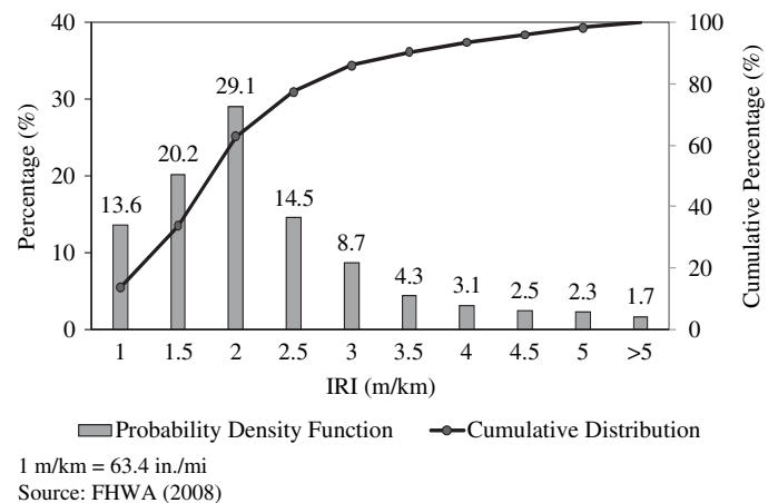
Figure 5-6. Road surface roughness distribution in the United States.
