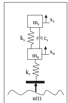
Figure 5-5. Parameters for quarter-car vehicle model.
