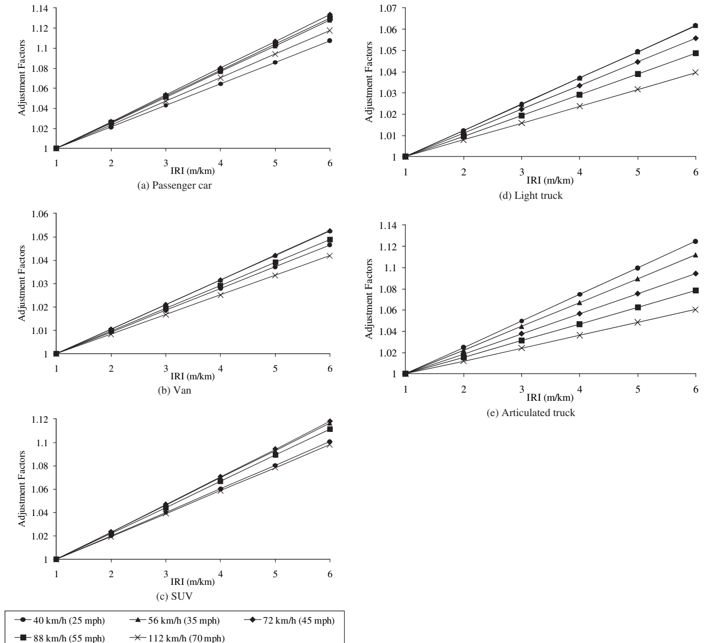
Figure 3-10. Effect of roughness on fuel consumption estimated using calibrated HDM 4.
