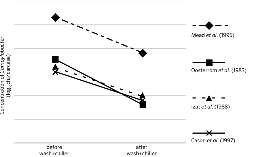
FIGURE 16. The effect of a selected slaughterhouse process on the Campylobacter concentration on chicken carcasses. The change in pathogen concentrations (expressed as log CFU per carcass) before and after the process is represented by a line connecting data points originating from the same study (adapted from Christensen et al. , 2001)
