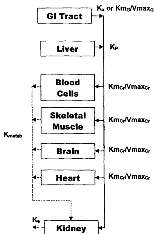
FIG. 5. Schematic of physiological model for creatine pharmacokinetics. Creatine enters the system through diet (first order rate constant K_a or Michaelis-Menten K_mG and V_{maxG} ) or zero-order hepatic production ( K_P ). K_mCr and V_{maxCr} represent Michaelis-Menten kinetics for saturable uptake of creatine by the creatine transporter. K_{METAB} is the first order rate constant for the conversion of creatine to creatinine. K_e is elimination rate constant for creatinine. Solid lines indicate the creatine pathway and dotted lines indicate the creatinine pathway. Values for rate constants: K_a or K_mG/V_{maxG} , none available; K_P = 1 g/day; K_{METAB} = 0.017 days; K_mCr/V_{maxCr} , see Table 1; and K_e = \text{GFR} .
