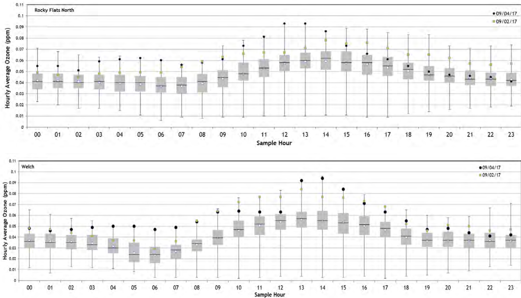
Figure 54: Diurnal Deviation from Normal Plots for hourly data at RFN (AQS ID 080590006) and Welch (AQS ID 080590005)
