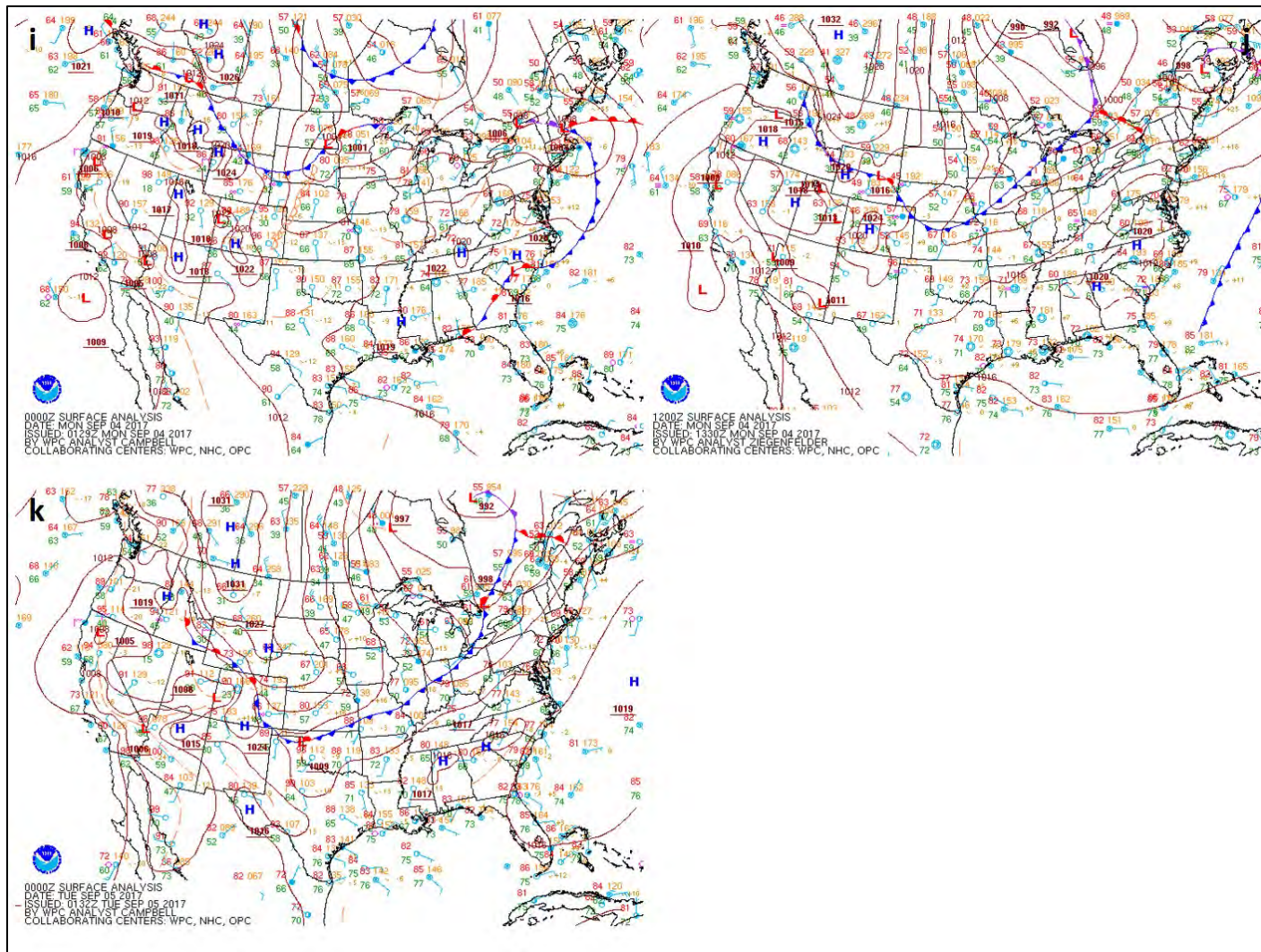
Figures 12i-k: NOAA surface analysis at (i) 5:00 PM MST (0Z September 4, 2017) September 3, 2017; (j) 5:00 AM MST (12Z) September 4, 2017; (k) 5:00 PM MST (0Z September 5, 2017) September 4, 2017. (source: http://www.wpc.ncep.noaa.gov/ )
