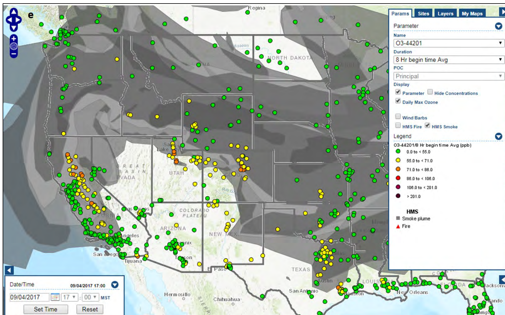
Figure 17e: HMS Smoke detection and 8-hr O 3 maximum concentration on September 4, 2017. (source: https://airnowtech.org/navigator )
