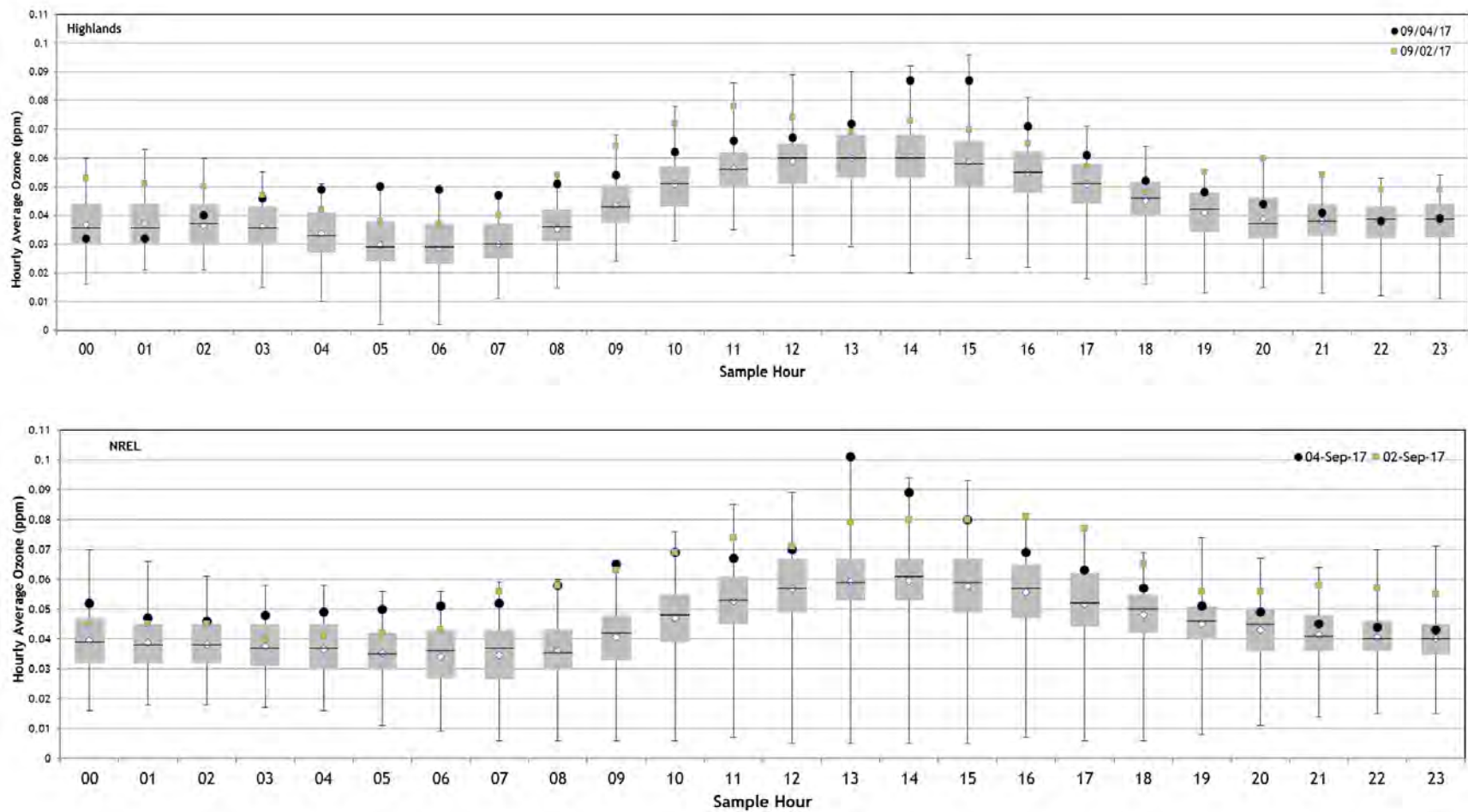
Figure 53: Diurnal Deviation from Normal Plots for hourly data at Highland (AQS ID 080050002) and NREL (AQS ID 080590011)
