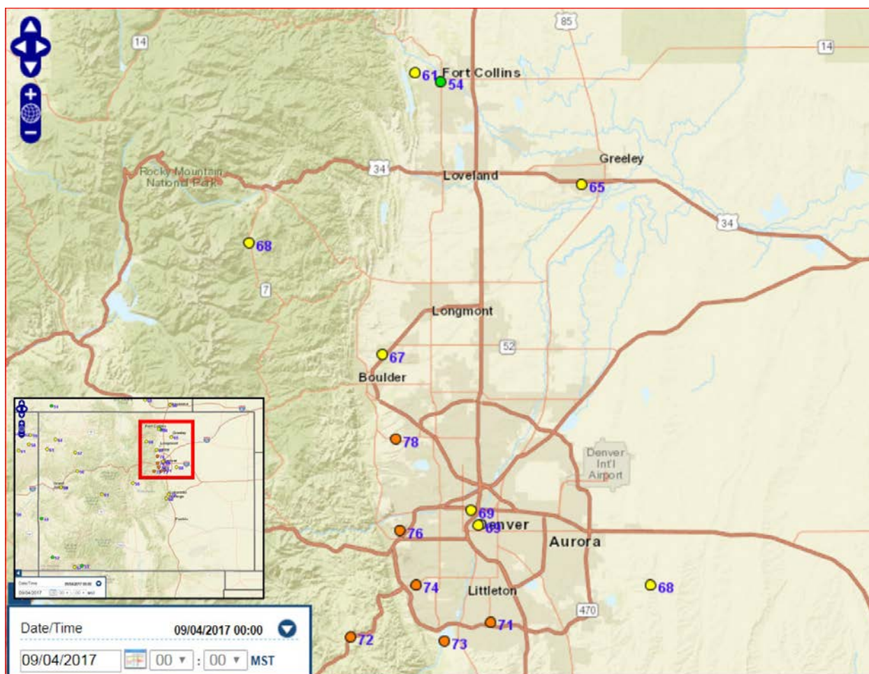
Figure 35: Maximum 8-hr average O 3 in ppb within the DM/NFR area on 9/4/2017, inset of the State of Colorado for geographical reference (source: https://airnowtech.org/navigator/ )
