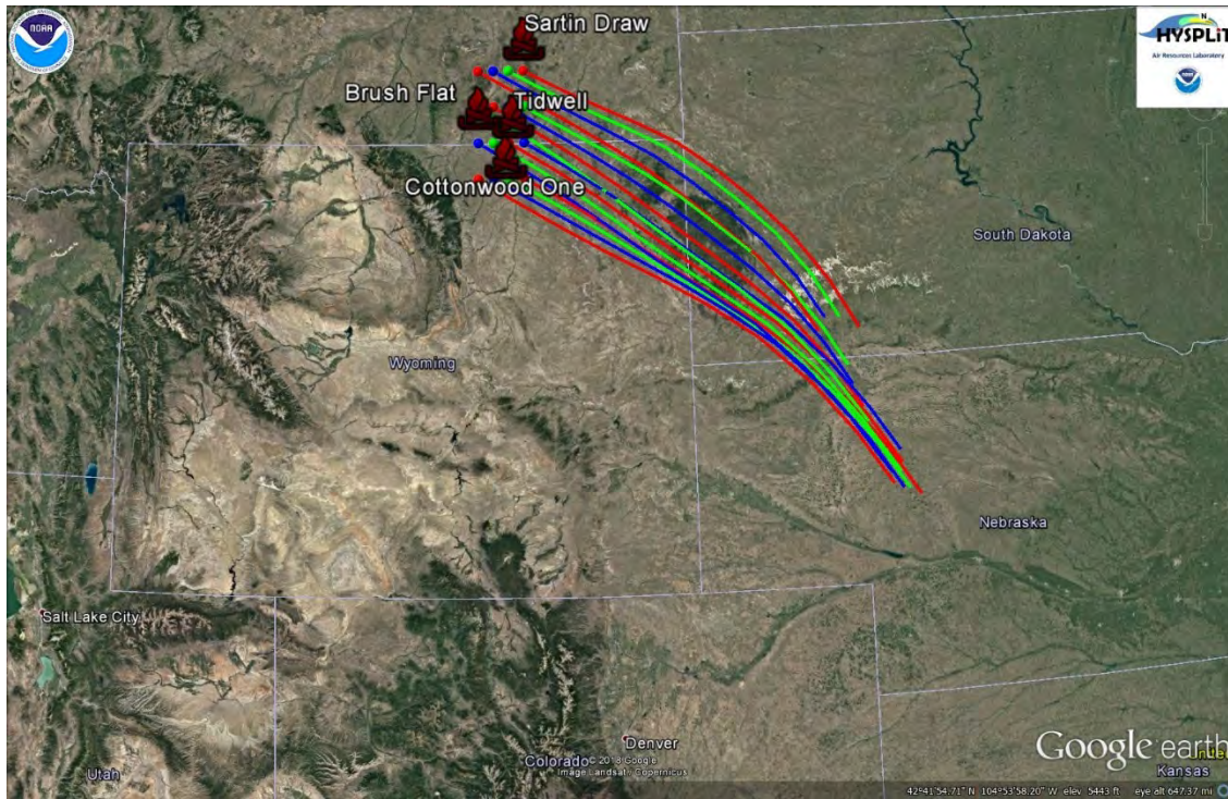
Figure 23: GDAS 9-hour HYSPLIT forward trajectory matrix from NE Wyoming/SE Montana wildfires at 2500 meters AGL, starting at 5 PM MST (0Z September 2, 2017) September 1, 2017 and ending at 2 AM MST (9Z) September 2, 2017. (source: https://ready.arl.noaa.gov/HYSPLIT.php )
