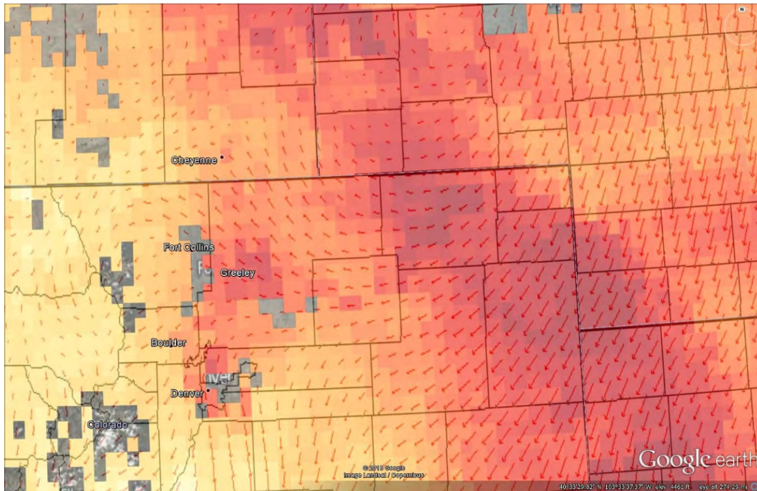
Figure 28: MODIS Terra AOD at approximately 11:12 AM MST (1812Z) and NAM Analysis wind vectors at 11:00 AM MST (1800Z) on September 2, 2017. (source: https://worldview.earthdata.nasa.gov/ )
