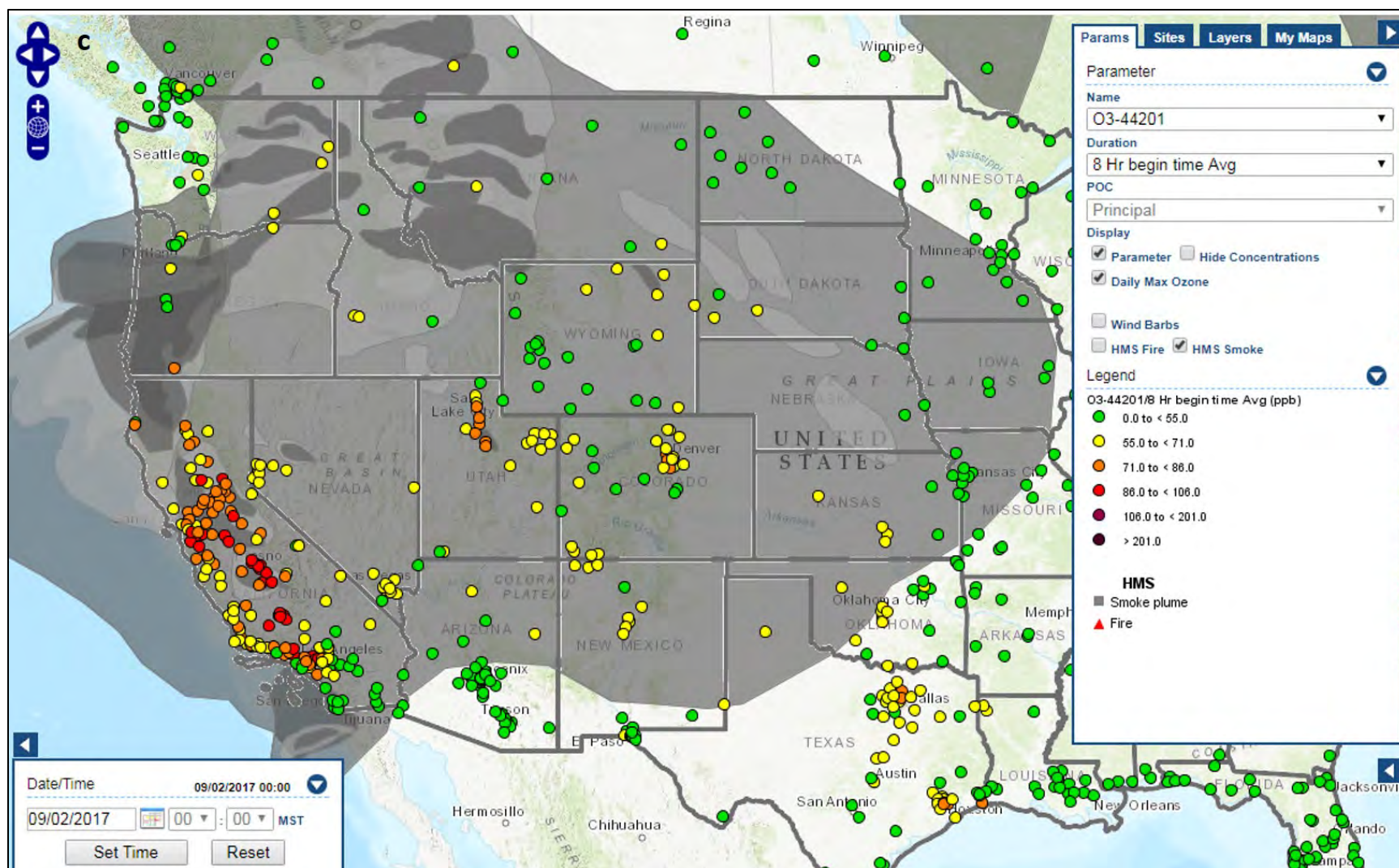
Figure 17c: HMS Smoke detection and 8-hr O 3 maximum concentration on September 2, 2017. (source: https://airnowtech.org/navigator )
