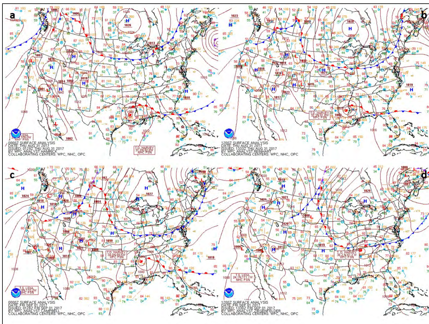
Figures 12a-d: NOAA surface analysis at (a) 5:00 PM MST (0Z August 31, 2017) August 30, 2017; (b) 5:00 AM MST (12Z) August 31, 2017; (c) 5:00 PM MST (0Z September 1, 2017) August 31, 2017; and (d) 5:00 AM MST (12Z) September 1, 2017. (source: http://www.wpc.ncep.noaa.gov/ )
