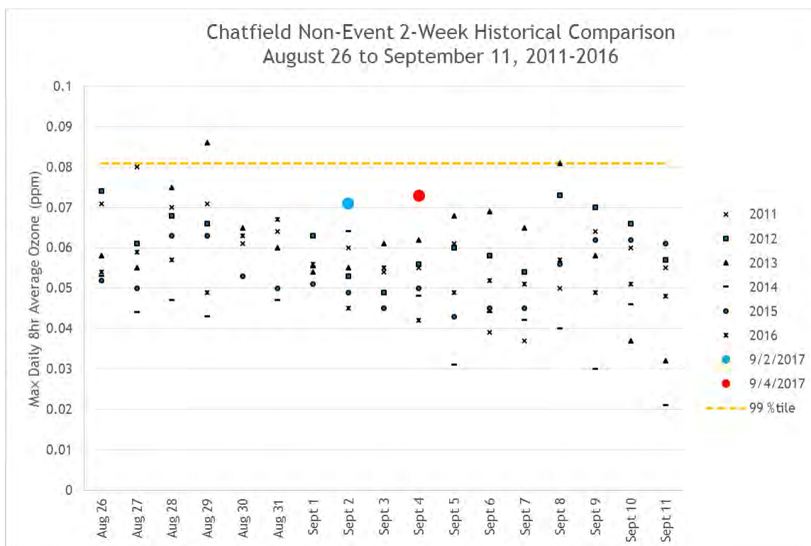
Figure 50: 2-Week Non-Event Historical Comparison Plots for Aspen Park (AQ5 ID 080590013) and Chatfield (AQ5 ID 080350004)
