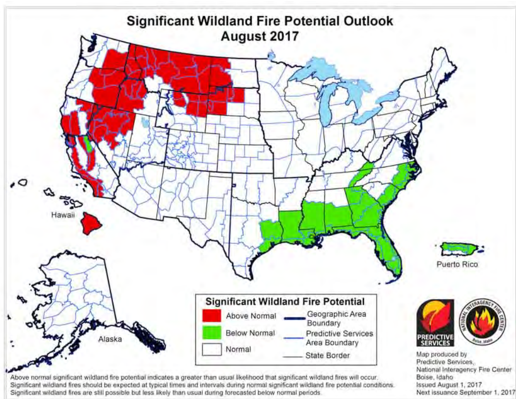
Figure 14: Significant Wildland Fire Potential Outlook for August 2017. (source: https://www.predictiveservices.nifc.gov )
