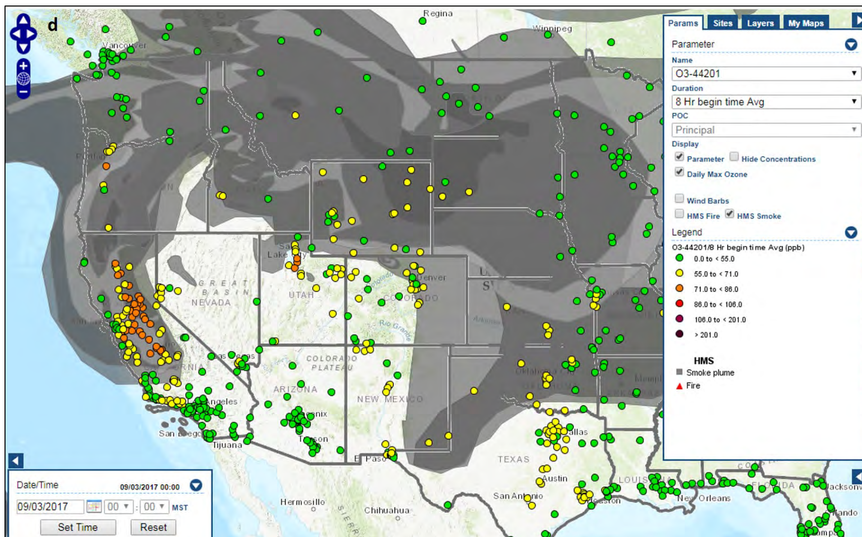
Figure 17d: HMS Smoke detection and 8-hr O 3 maximum concentration on September 3, 2017. (source: https://airnowtech.org/navigator )
