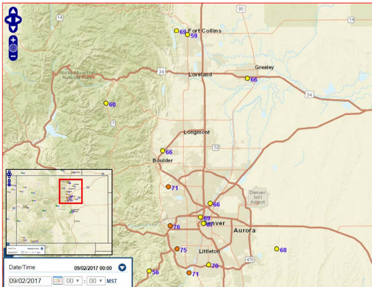
Figure 20: Maximum 8-hr average O 3 in ppb within the DM/NFR area on 9/2/2017, inset of the State of Colorado for geographical reference (source: https://airnowtech.org/navigator/ )
