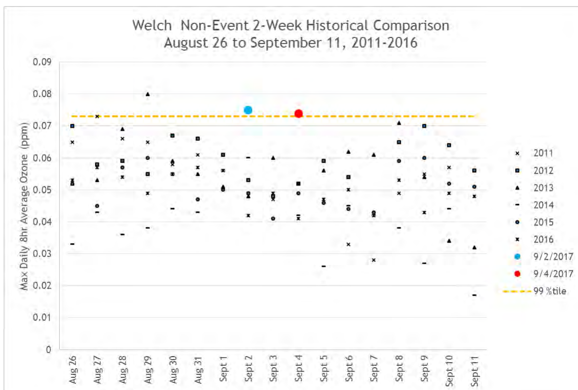
Figure 52: 2-Week Non-Event Historical Comparison Plots for RFN (AQ5 ID 080590006) and Welch (AQ5 ID 080590005)
