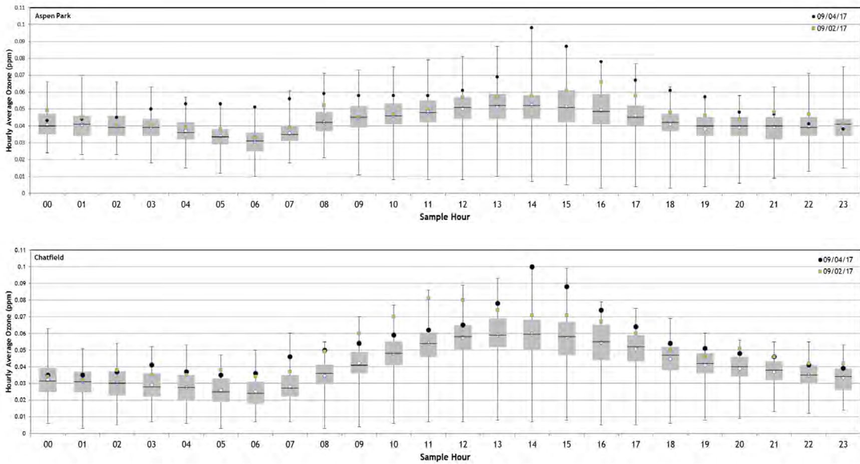
Figure 53: Diurnal Deviation from Normal Plots for hourly data at Aspen Park (AQ5 ID 080590013) and Chatfield (AQ5 ID 080350004)
