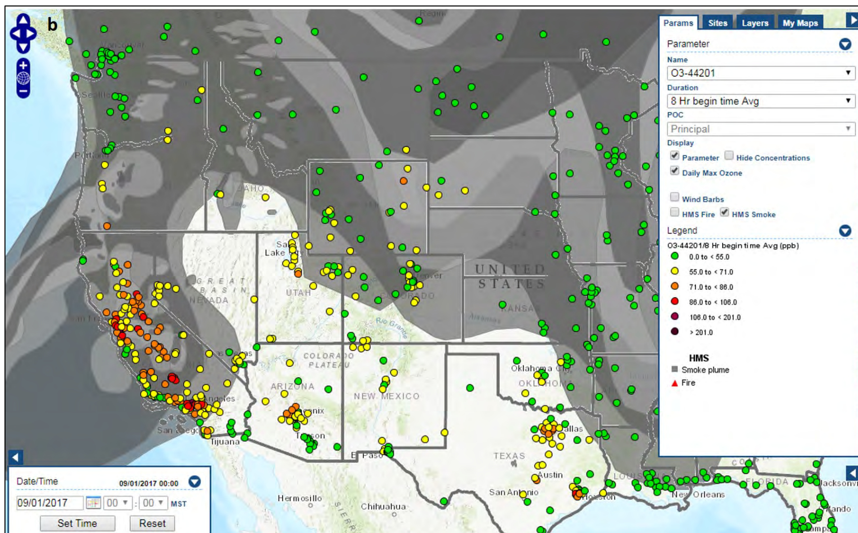
Figure 17b: HMS Smoke detection and 8-hr O 3 maximum concentration on September 1, 2017. (source: https://airnowtech.org/navigator )
