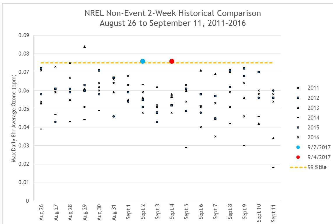
Figure 51: 2-Week Non-Event Historical Comparison Plots for Highland (AQ5 ID 080050002) and NREL (AQ5 ID 080590011)
