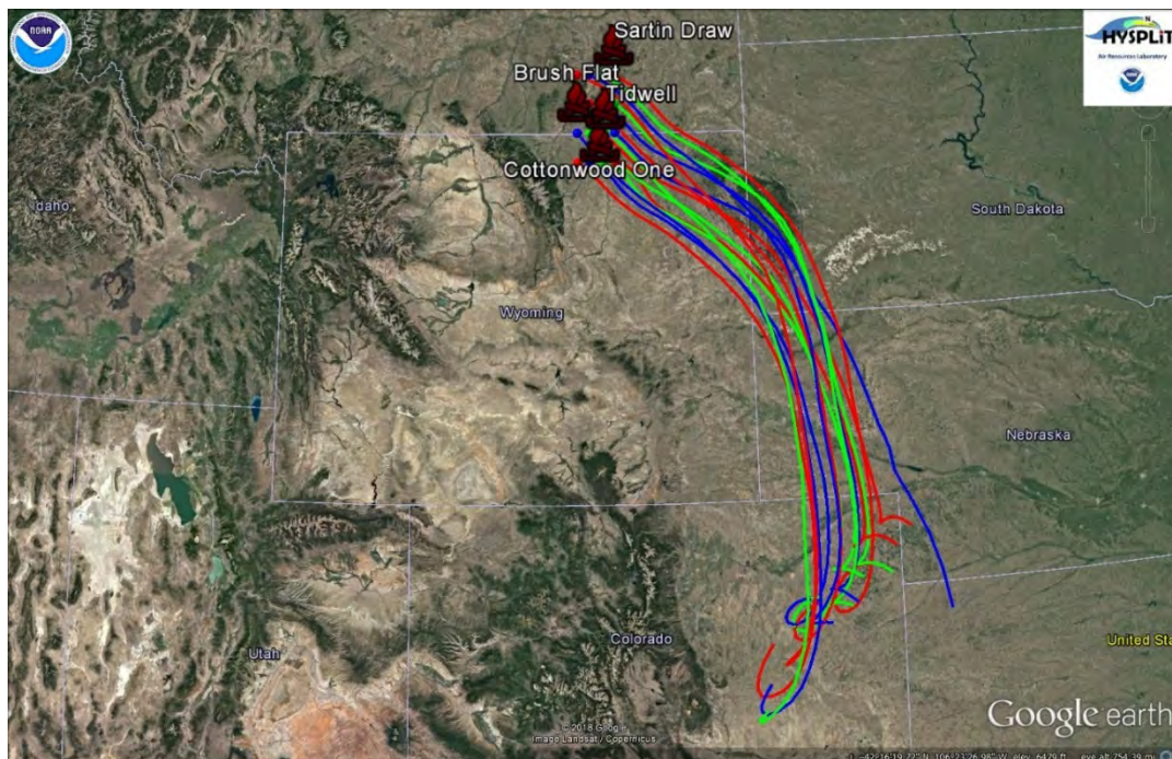
Figure 22: GDAS 33-hour HYSPLIT forward trajectory matrix from NE Wyoming/SE Montana wildfires at 2500 meters AGL, starting at 5 PM MST (0Z September 1, 2017) and ending at 2 AM MST (9Z) September 2, 2017. (source: https://ready.arl.noaa.gov/HYSPLIT.php )
