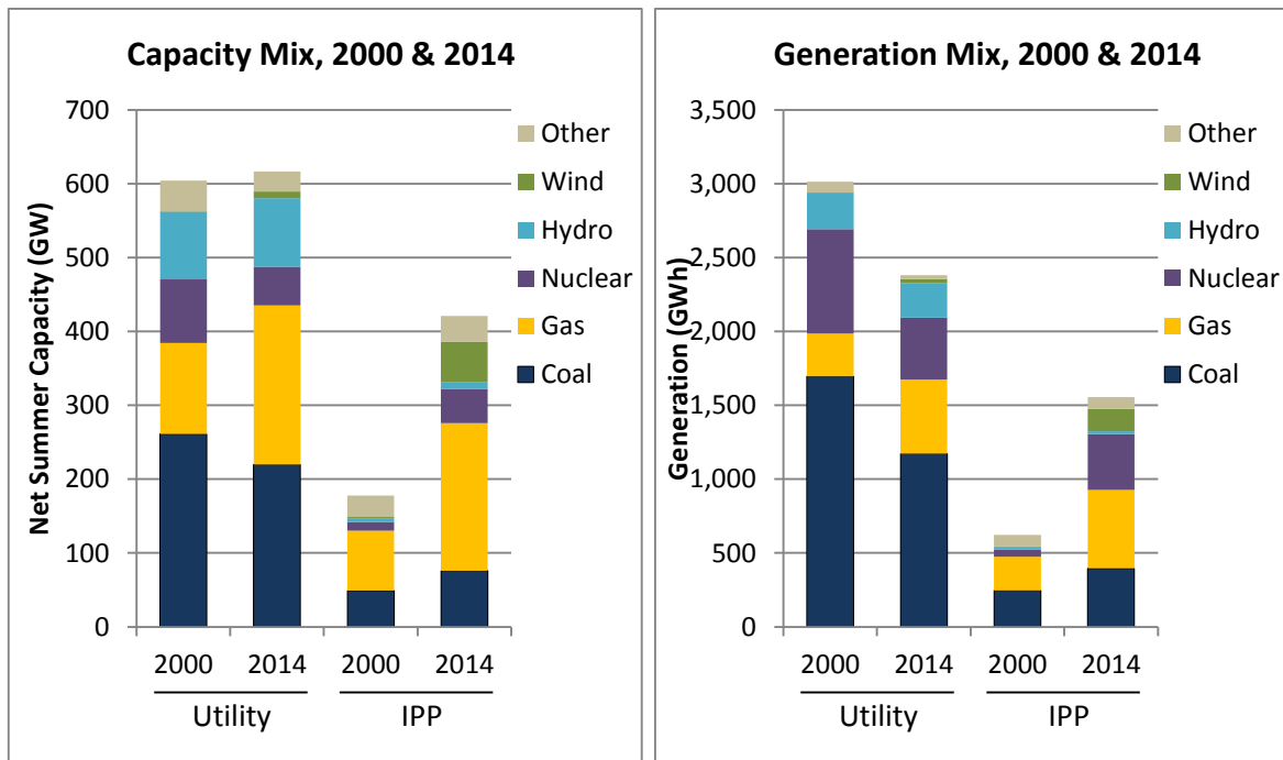
Figures 2-13 & 2-14. Capacity and Generation Mix by Ownership Type, 2000 & 2014
