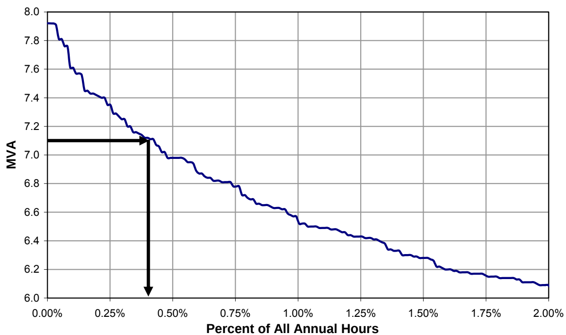
Figure 23. Portion of load duration curve with highest values.
