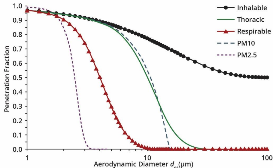
Figure 2–5. Reproduced from NIOSH [2024b]. The inhalable, thoracic, respirable, PM 10 , and PM 2.5 particle penetration curves
